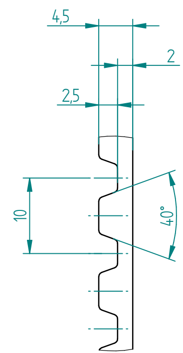
DETAIL C SCALE 2:1
