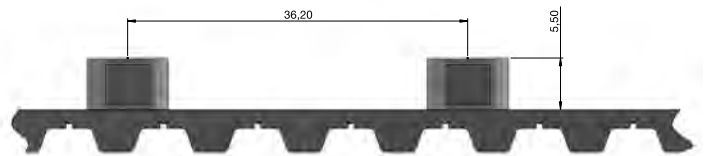
EBMI000006 PU Molded 26 T10 3040 Steel + 84 Cleats Sidecut
