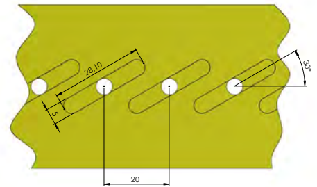
EBPU000398 | EBP000397 PU 50T10-920 Aramid NC + PUC060 Yellow
